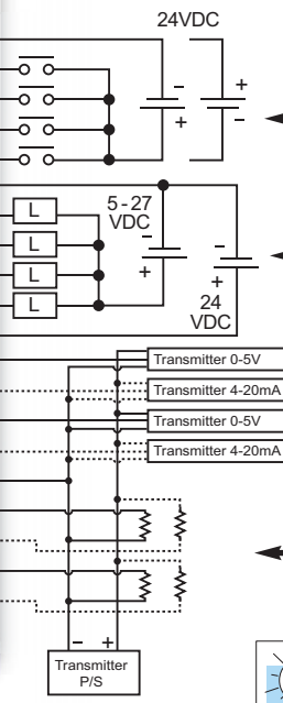
Wiring Diagram
