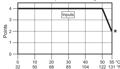
C0-02DR-D Temperature Derating Chart
