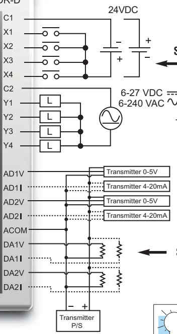
Wiring Diagram
