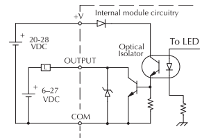
Equivalent output circuit Standard output (Y2-Y17)
