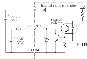
Equivalent output circuit Pulse output (Y0-Y1)
