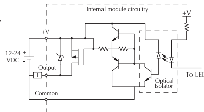
Equivalent output circuit Pulse output (Y0-Y1)
