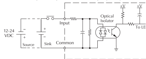
Equivalent input circuit, Standard inputs (X4-X23)
