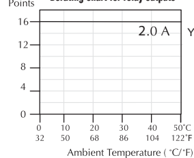
Derating chart for relay outputs
