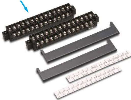
DL06 replacement terminal blocks, terminal block covers, terminal block labels and short bar D0-ACC-2
