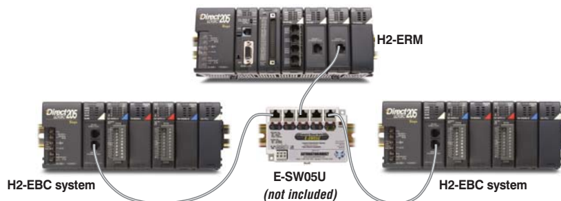
Example of an Ethernet remote I/O system using an H2-ERKIT-2. CPU, bases, I/O modules, Ethernet switch, etc. are sold separately.
