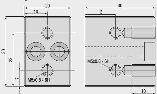
mounting block
